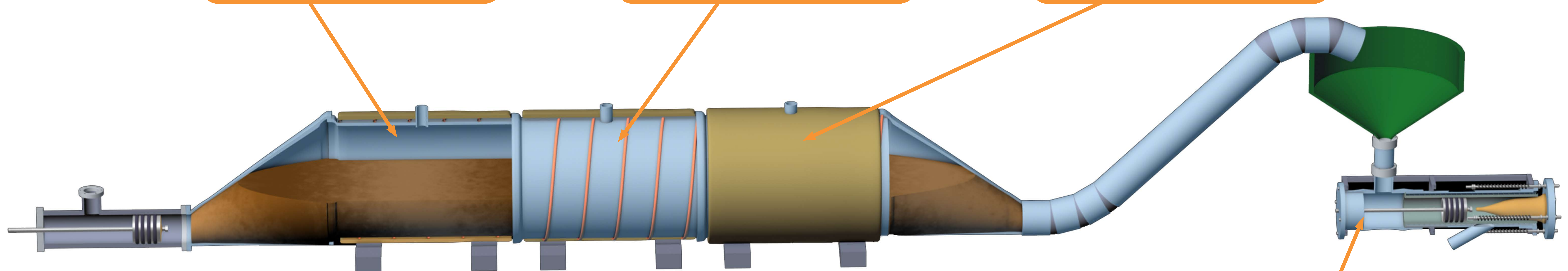
The complete Avatar Digester. This cross view shows the piston pump injection of manure through processing to separator.
